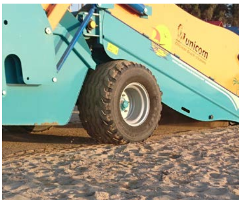
Special wheels for the beach. They guarantee a good floatability on the sand and bring a strong traction.
