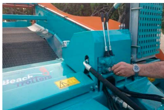
Control levers of the mesh and the frontal roller
